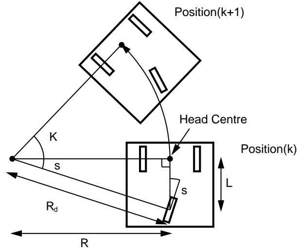
Figure 3.7: With the angle of the vehicle's single rear steering wheel set to s(k) , the "head centre", lying centrally above the fixed axis of the front wheels, moves in a path of radius R(k) = L/\tan(s(k)) . L is the vehicle's constant wheelbase.
