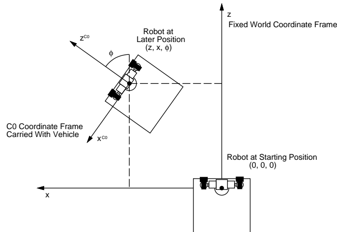
Figure 3.6: The vehicle’s location in the world coordinate frame is specified with the coordinates (z, x, \phi) . The C0 coordinate frame is carried with the vehicle.
