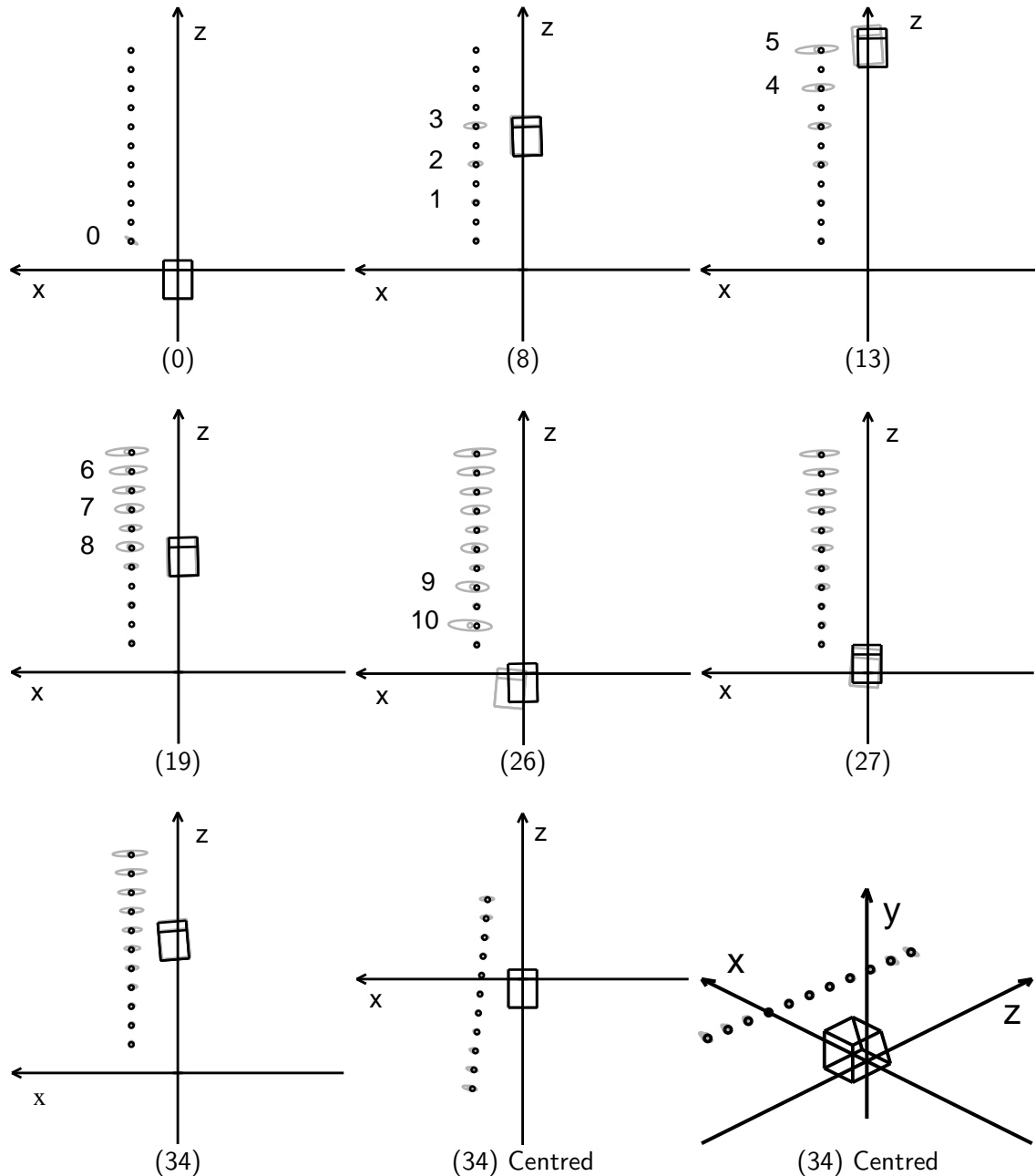
Figure 5.12: Steps from experiment C1 using fully coupled robot and feature estimates.
