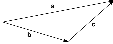
Figure 3.1: The vector sum \mathbf{a} = \mathbf{b} + \mathbf{c} .
