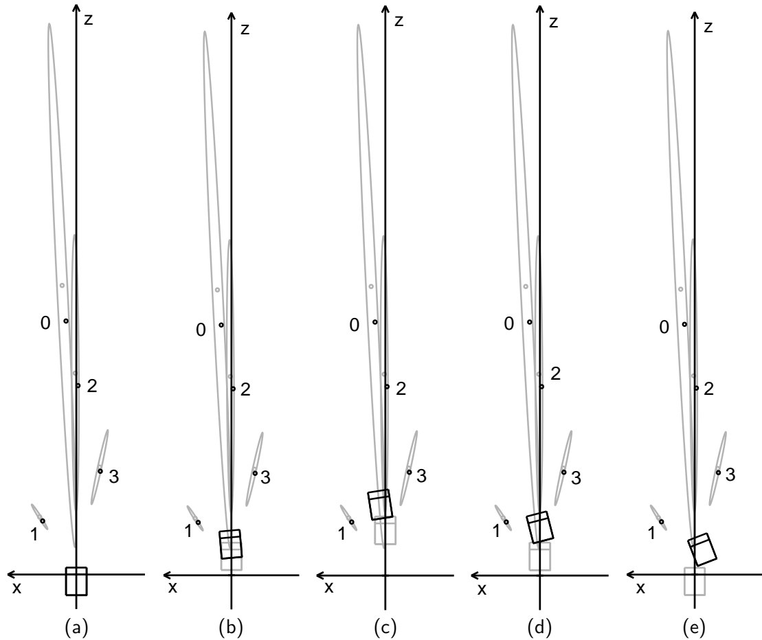
Figure 5.4: Estimating robot position using odometry only in experiment A1: grey shows system estimates of robot and feature locations, and black the actual measured values. From its starting position at (a) the robot moves forward through (b) to its most advanced location at (c), before reversing back through (d) to (e). It can be seen that the robot position estimate quickly diverges from the ground-truth due to poor odometry calibration.
