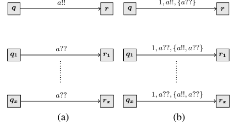
Figure 1: Simulation of broadcast protocols by PCGS.
