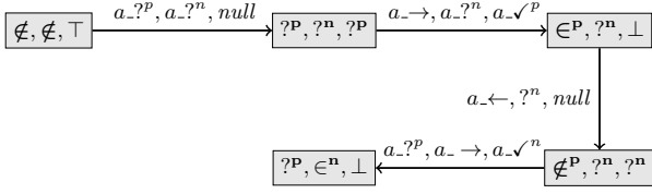
Figure 4: Fragment of the CCGS \mathfrak{G}((1, 1)) .
