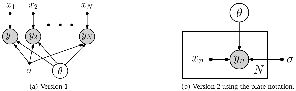
Figure 1.14: Two graphical models for linear regression. Observed random variables are shaded, deterministic parameters are dots. (a) Graphical model without plate notation; (b) Graphical model with plate notation, which allows for a more compact representation than (a).
