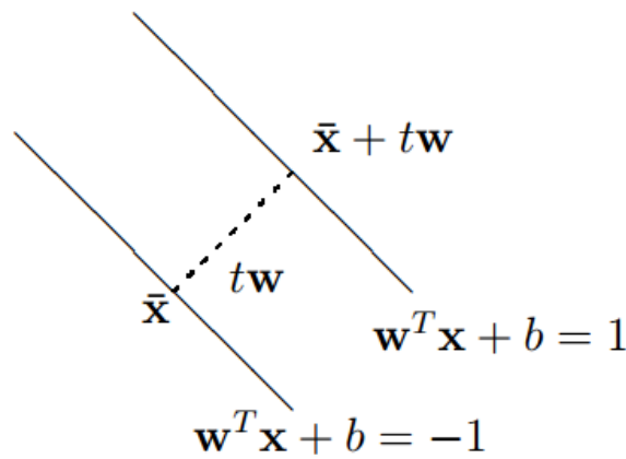
Figure 3.1: Separating Hyperplanes.
