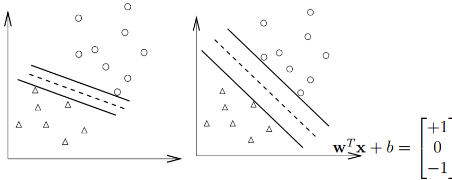
Figure 3.1: Separating Hyperplanes.
