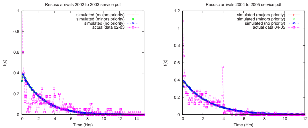
Figure 4.7: Actual and simulated service time density for blue call arrivals using 2002/2003 data (left) and 2004/2005 data (right).
