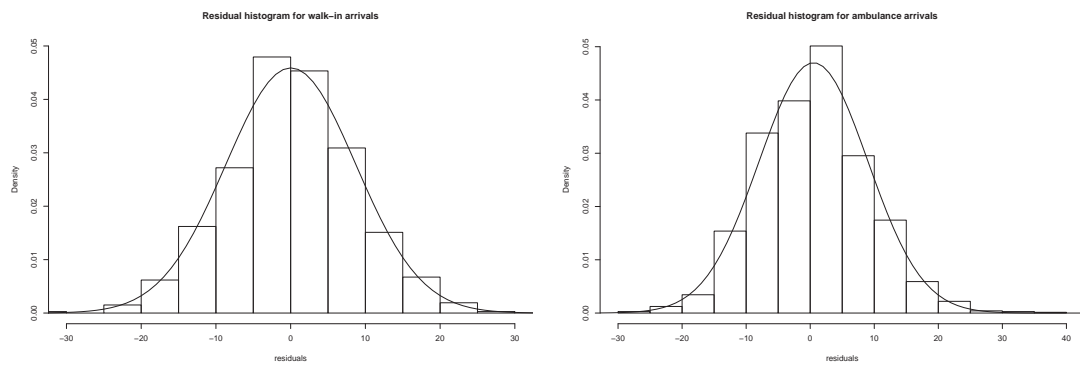
Figure 3.22: The distribution of the residuals of the ST models of walk-in (left) and ambulance (right) arrivals and the corresponding normal distributions.
