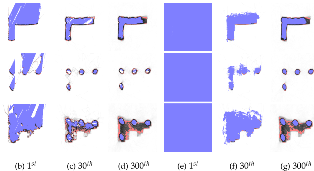
Figure 7.15: Complete reconstruction of the Middlebury temple model performed on the full dataset (a). We illustrate the volume slices from which the volumetric SDF evolution is tracked in figures (b-d) and (e-g), where each plane (top, middle, bottom) is associated with the slices (1,2,3). In (b-d) we show the TSDf evolution where freespace is shown in blue which zero level set show in red. (b) Shows the result after integrating 1 depth map, followed by (c) 30 depth maps and (d) shows the near complete model with 300 depth maps integrated out of 312. (e-g) show the equivalent evolution using confidence thresholding of the voxel weight function \mathcal{W}_r . Confidence based thresholding results in a more conservative estimate of the known surface location used in model prediction as described in Subsection (7.4.3). We will also make use of the conservatively estimated geometry in the dense frame-model camera tracking method detailed in Chapter (8).
