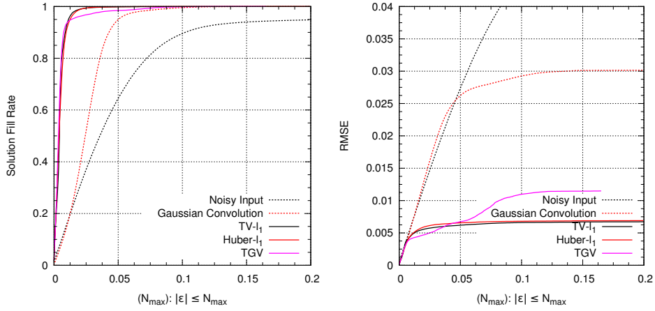
(a) Solution fill rates.
