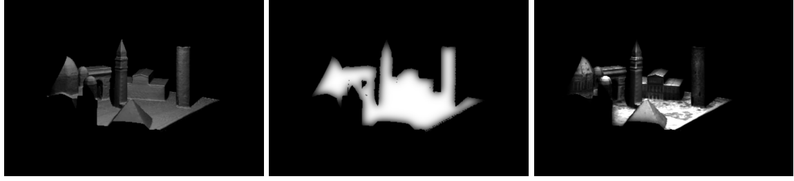
(a) Surface visibility weight: v_{sk} (b) Feathered pixel validity mask: b_{sk} (c) View dependent texture for novel view s .
