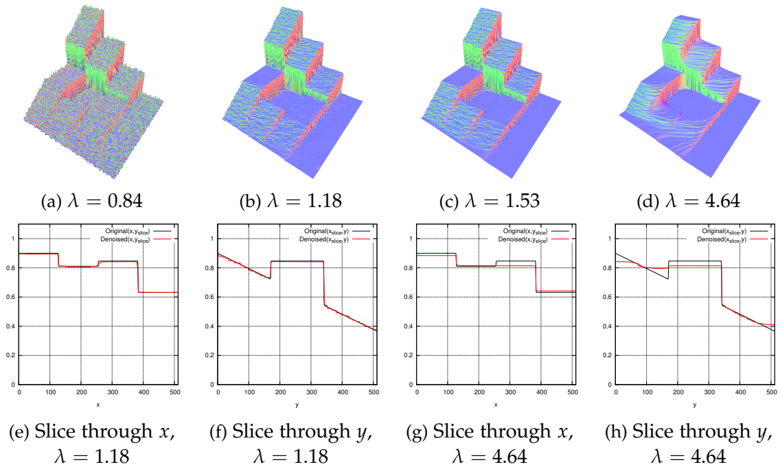
Figure 4.8: TV-\ell_1
