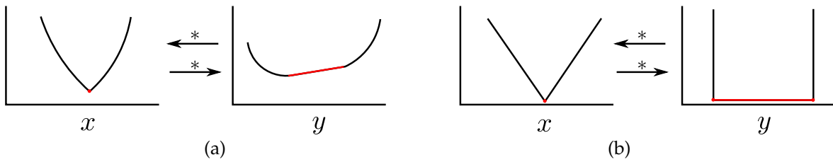
Figure 3.3: The Legendre-Fenchel transform takes non-differentiable points in F(x) to affine sections in F^*y . Figure adapted from Touchette (2005) , an accessible introduction to the convex conjugate. In (a) and (b) non-differentiable points are transformed to affine regions in the functions conjugate. In (b) the \ell_1 function is transformed to the indicator function.
