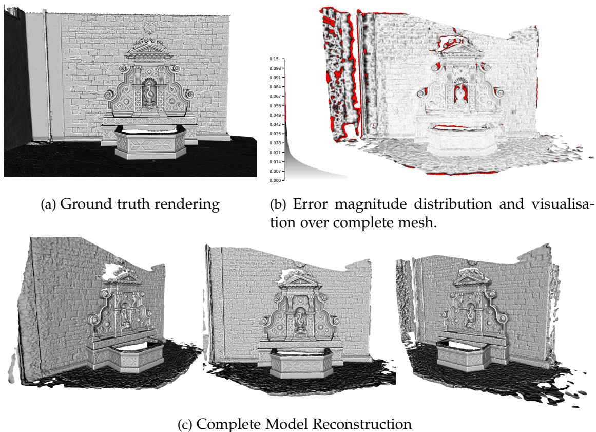
Figure 5.13: Reconstruction of the complete fountain-P11 scene using 7 depth maps. Fusion of the individual depth maps is performed using Poisson surface reconstruction with default settings and maximum octree depth 10, followed by removal faces with connected edges greater than 0.2m . We compute the absolute error over the entire model (b) against the ground truth rendered in (a), using the Hausdorff distance. The absolute error histogram is shown in meters, note that the error range is halved to [0 - 0.05]m encoded from white to black grey scales to enable greater inspection of errors on the complete model; red pixels show error magnitude above 0.05m .
