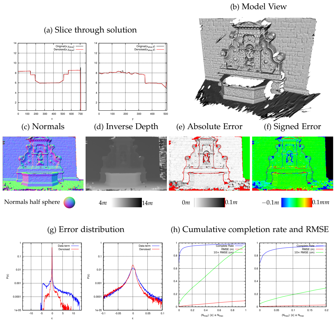
Figure 4.18: TGV_{\alpha}^2 - \ell_1 Solution, \lambda = 1.667 .
