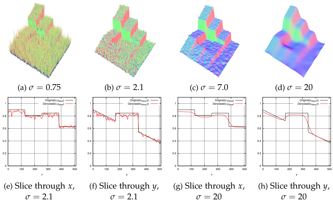
Figure 4.6: Gaussian Convolution
