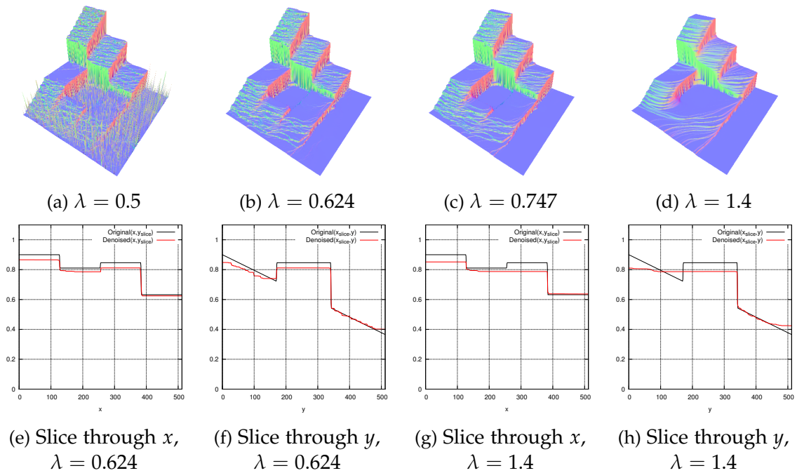
Figure 4.7: TV-\ell_2^2
