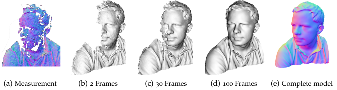
Figure 1.12: Example reconstruction using the truncated signed distance function averaging approach. (a) Shows the set of vertices computed from one depth image captured from a commodity structure light camera, rendered to show the surface normal orientation. In (b,c,d) the partially reconstructed surface is shown with Phong shading, computed from 2, 30 and 100 calibrated surface observations of the subject acquired from a moving sensor. The complete model from approximately 20 seconds of modelling is shown in (e), rendered into the same camera pose as from measurement (a) highlighting the denoised and filled in reconstruction obtained.
