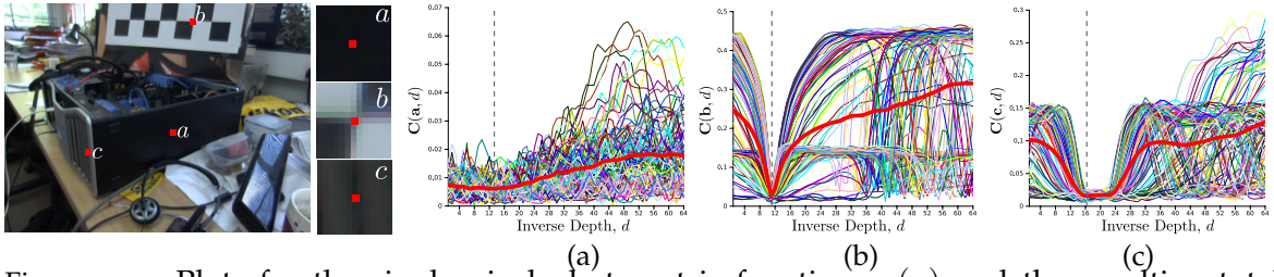
Figure 5.4: Plots for the single pixel photometric functions \rho(x) and the resulting total data cost row \mathbf{C}(x) are shown for three example pixels in the reference frame, chosen in regions of differing discernibility. Pixel (a) is in a textureless region and not well localisable; (b) is within a strongly textured region where a point feature might be detected; and (c) is in a region of linear repeating texture. While the individual costs exhibit many local minima, the total cost (thick red line) shows clear a clear minimum in all except for nearly homogeneous regions.
