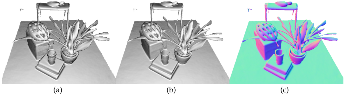
Figure 6.5: Rendering of a reconstructed scene with raycasting of the TSDF. In (a) the basic raycasting result is shown using trilinear interpolation of the TSDF function. In (b) we show the same ray-casting solution but using the analytical zero crossing intersection resulting in higher quality surface boundaries using Equation (6.22). The normal map rendering for the scene is shown in (c).
