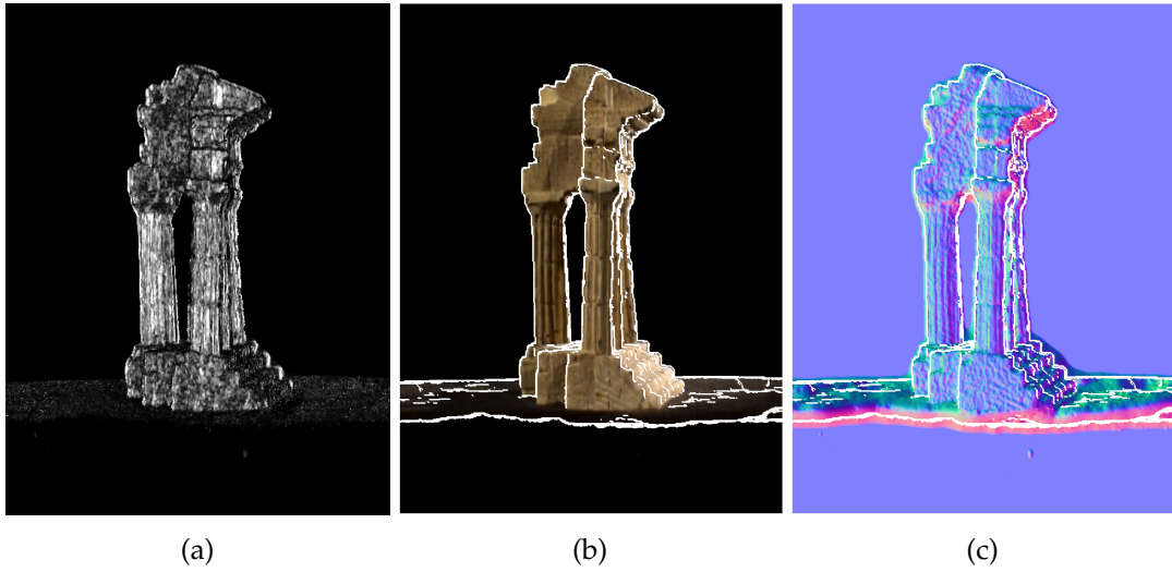
Figure 7.12: Depth map uncertainty (a) and normal map estimate (c) which together with the depth map estimated for the reference frame (b), and used in the TSDF fusion. We note that culling of estimated values with reduced visibility results shown on the reference frame (b) results in the removal of potentially valid estimated depth map values.
