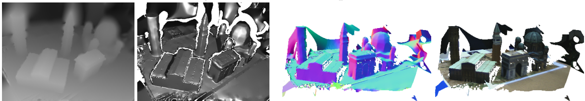
(c) \text{TGV}_\alpha^2\text{-}\ell_1 , linearised patch.
