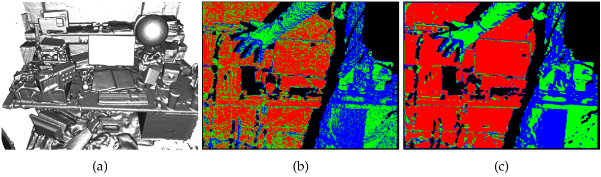
Figure 8.5: Example of point-plane outliers as person steps into a partially reconstructed scene shown rendered in (a). Outliers from compatibility checks (Equation 8.33) using a metric surface measurement from Kinect (b). \Omega(u) \neq \text{null} are shown in red, V_l(u') are shown in black and outliers are shown for incompatibility in normal (green) and both distance and normal (blue). In (c) we demonstrate the improved data association by performing tracking on a bilateral-filtered version of the raw depth map used in the KinectFusion application described in Chapter (9).
