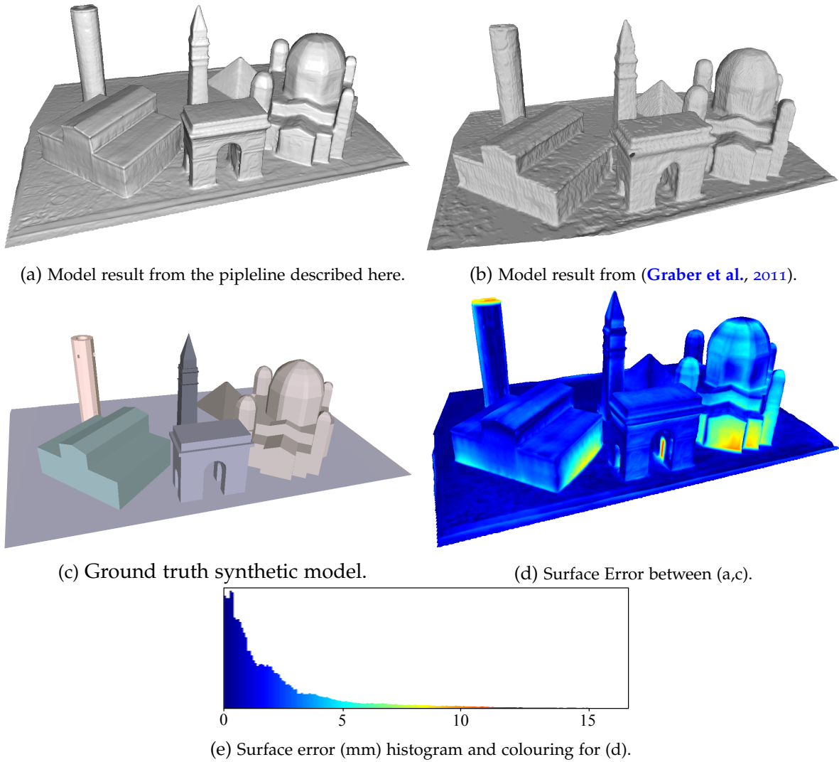
Figure 7.19: Reconstructing the City of Sights from Gruber et al. (2010). (a) Reconstruction from the pipeline described in this Chapter. (b) Result from Gruber et al. (2011). (c) Virtual ground truth model. (d) Error surface visualisation between (a) and (c). (e) Error histogram with associated colour key for the surface error in (d), ranging from 0mm - 17mm error, quantised into 256 bins. We note that the cited root mean square error for the constructed paper model relative to the ground truth is approximately 3mm (Gruber et al., 2010).
