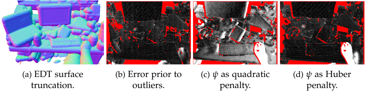
Figure 8.7: Example tracking using the true distance field computed using the EDT on an office desktop scene. In (a) we render the scene showing the level set of the distance field at approximately 30mm truncation, resulting in the blob like appearance of the modelled objects. In (b) we show an example error image in the live frame, prior to motion of hand and arm shown in the bottom right corner of the reconstruction: red pixels indicate no valid surface measurement while the intensity of the remaining pixels indicate the absolute error computed in Equation (8.38). In (c,d) a hand in the scene moves presenting outliers to the static scene. In (c) the use of a quadratic penalty term results in a biased solution, while in (d) the Huber penalty is capable of down-weighting the outliers resulting in the correct pose estimate.
