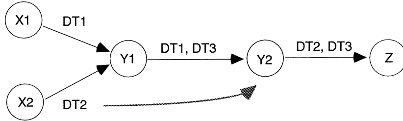
Figure 5.3 Misuse of Delegation Token if PDT field is omitted
