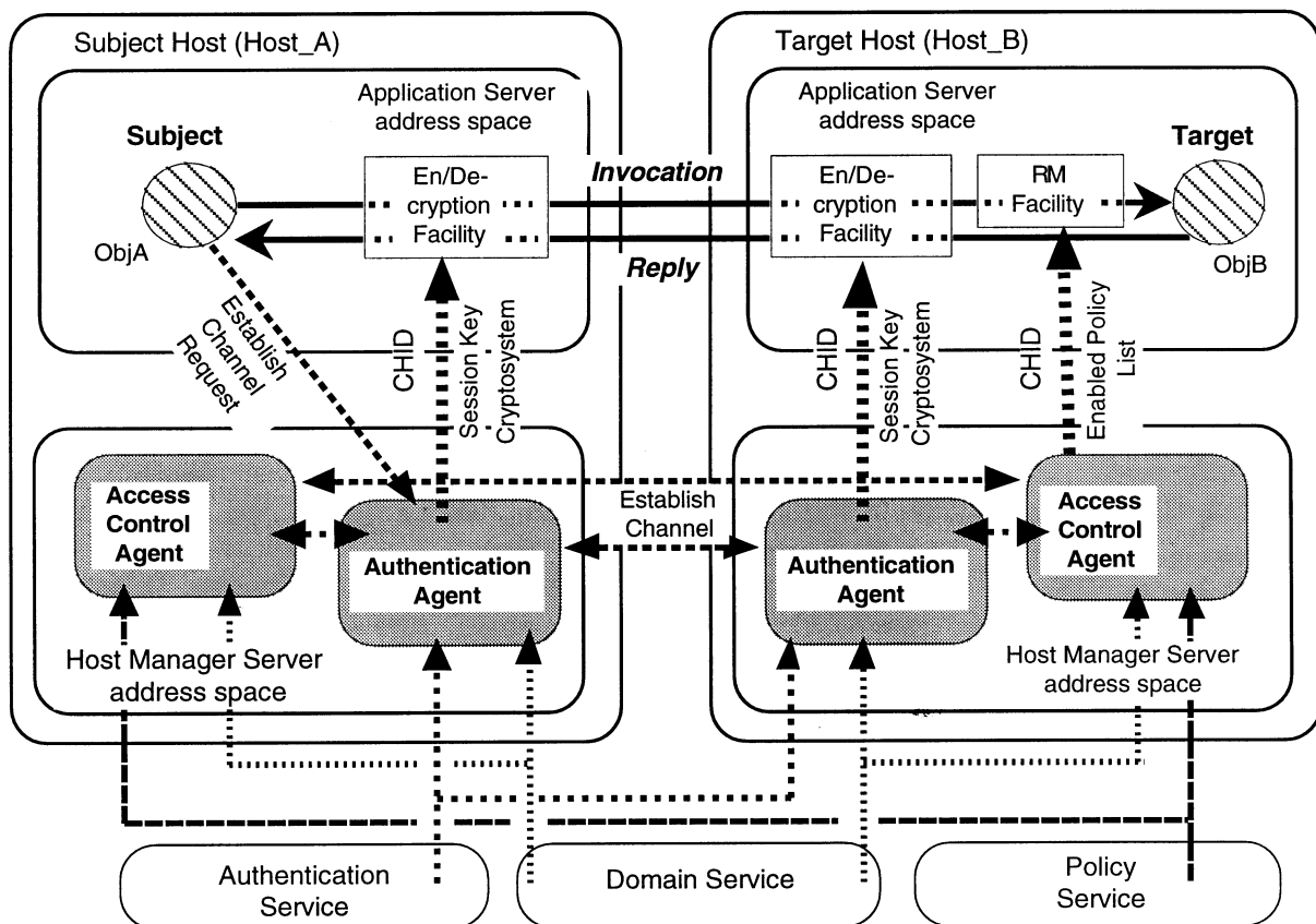
Figure 3.2 Basic Security Architecture
