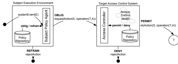
Figure 5: Policy enforcement model
