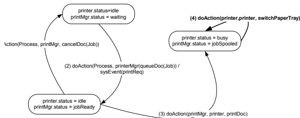
Figure 4: State chart for Printer system functionality.
