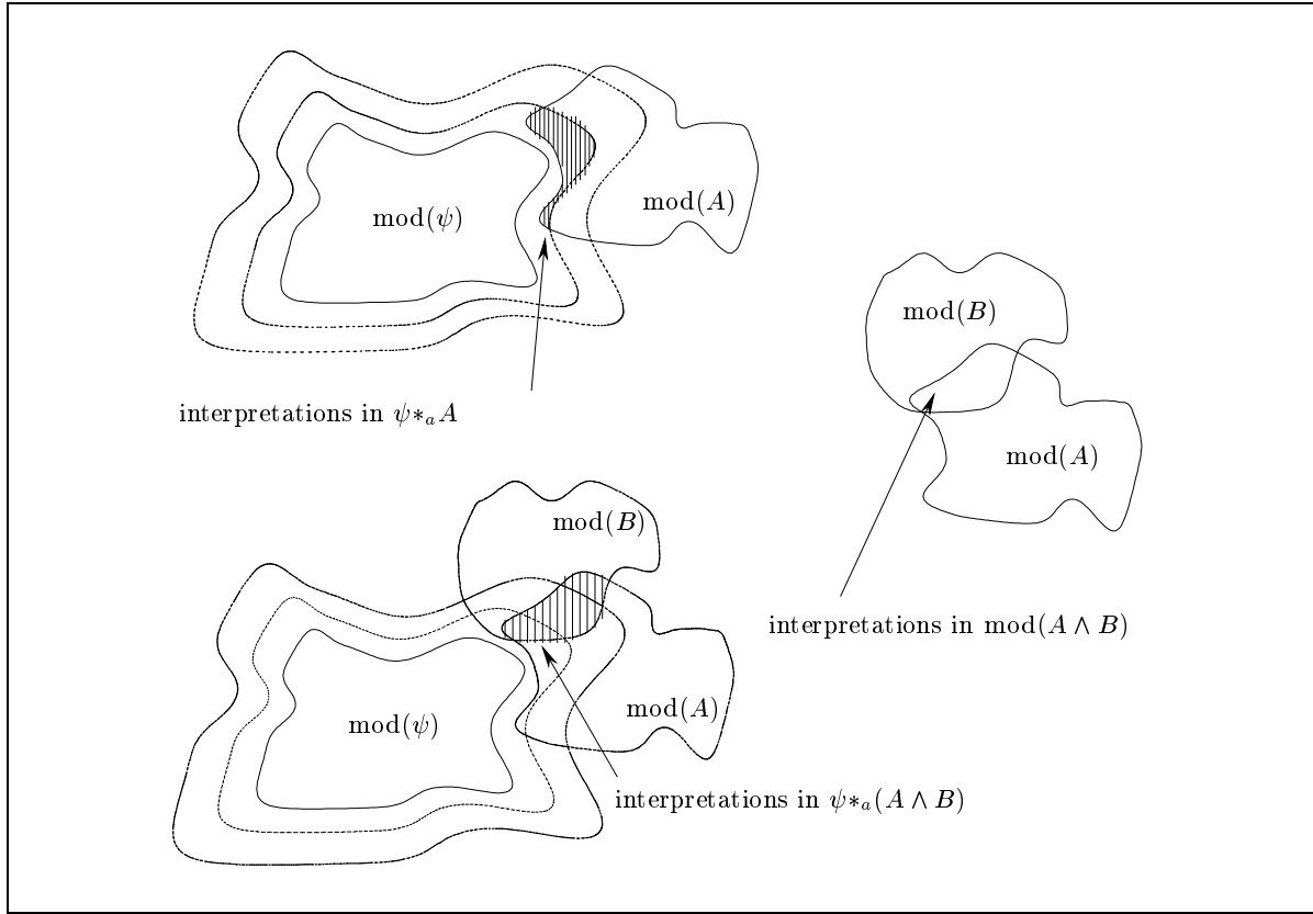
Figure 1: Illustrating postulate (K*8).
