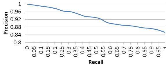
(b) p = 3.15 and N = 100
