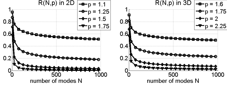
Figure 3: Choosing N : The figures plot the residual ratio R(N, p) versus N for different p values in 2D (left) and in 3D (right). As expected the error upper bound drops with increasing N . The rate of decrease also becomes faster with increasing p . This inverse relation suggests the trade-off between N and the sensitivity of WESD to finer scale shape differences since WESD becomes less sensitive as p increases, see Section 3.3.
