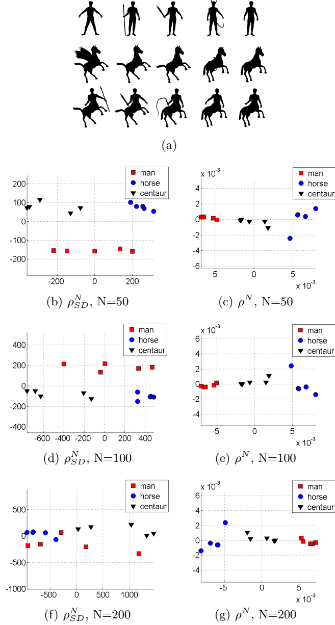
Figure 5: Low dimensional embeddings: (a) The 15 objects used in this experiment. The graphs plot the 2D embeddings of the objects based on the affinity matrices constructed by \rho_{SD}^N and WESD ( \rho^N ). Each row presents the results based on different number of eigenvalues: 50, 100 and 200 from top to bottom respectively. The structures of the 2D embedding based on \rho_{SD}^N are quite different for different N . WESD however, produces embeddings that are similar. This demonstrates the stability of the embedding with respect to N when WESD is used.
