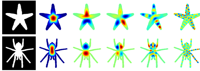
Figure 1: Starfish and tarantula. The objects represented as binary maps are shown on the left, followed by the 1st, 2nd, 5th, 20th, and 100th eigenfunction. The values increase from blue (negative) to red (positive) with green being zero.
