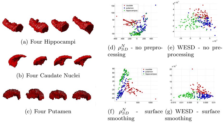
Figure 7: 2D embedding of subcortical structures: 240 structures (80 caudate nucleus, 80 putamen and 80 hippocampus) are extracted from MR scans of 40 different individuals. (a),(b) and (c) show some example structures from this dataset. Note the high intra-class variability and the artefacts due to finite resolution and manual segmentations. (d) and (e) plot 2D embeddings of these 240 structures obtained based on the affinity matrices computed via \rho_{SD}^N and WESD respectively. These embeddings are computed without any preprocessing applied to the structures. The embedding obtained with WESD distinctly clusters the objects with respect to the anatomical structures. The embedding in (d) however, shows some ambiguities in the separation. Graphs in (f) and (g) plot the similar embeddings obtained after smoothing the surfaces of the structures to remove artefacts. The embedding obtained by \rho_{SD}^N , although better than (d), still suffer from similar problems. The embedding based on WESD on the other hand, now even between better separates the groups.
