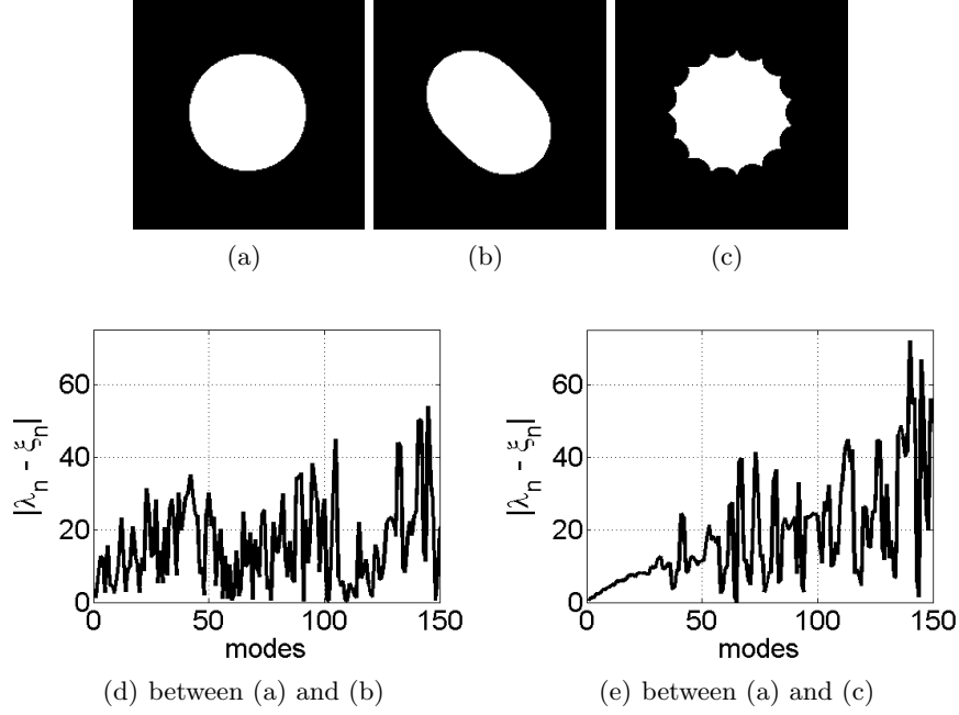
Figure 2: Multi-scale characteristics of different spectral modes: (a), (b) and (c) show three synthetic shapes. In (d) we plot the absolute differences between the corresponding modes of (a) and (b) with respect to the spectral index. In (e) we plot the same difference for the shapes in (a) and (c). The shape difference between (a) and (b), which is at a coarser level, is already captured at the lower spectral modes. The difference between (a) and (c) results in lower differences in lower spectral modes because these objects are more similar at a coarser level. At the higher spectral modes though the difference between (a) and (c) becomes more prominent since these objects differ more substantially at the finer scales. The plots in (d) and (e) demonstrate that the higher modes for a given object are more important for finer scale shape details.
