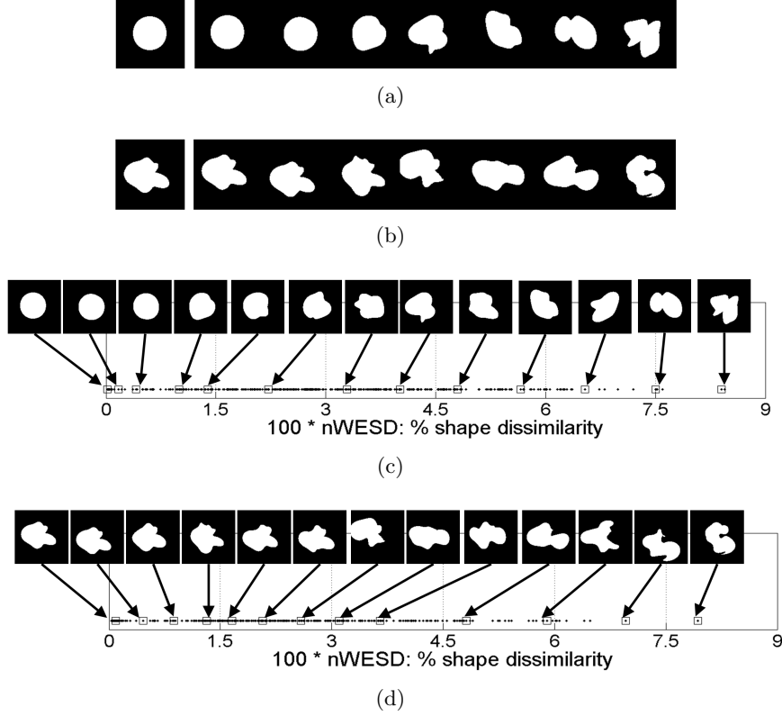
Figure 4: Shape-based ordering of objects: We generate two artificial datasets each consisting of a reference object and its random deformations. Samples from the datasets are shown in (a) and (b). The binary images to the very left show the reference objects for each dataset. We then ordered all the deformed objects with respect to the nWESD scores between the object and the reference. The graphs in (c) and (d) plot these orderings. Based on visual inspection the ordering is quite reasonable.
