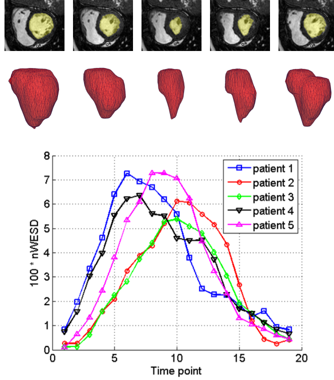
Figure 8: Analysing 3D + time (4D) cardiac images: Top row shows corresponding 2D slices of a 4D MRI dataset at time points t = \{0, 3, 6, 9, 12\} . In the middle row, 3D shapes extracted at each of the time points. For five patients, we compute the nWESD shape dissimilarity score of the LV blood pool at each time point with respect to its shape at t = 0 . The graph plots these scores. We note that the proposed shape distance is able to capture the dynamic process of the LV shape changes and furthermore, the symmetry between the two phases of an heart beat: diastole and systole.
