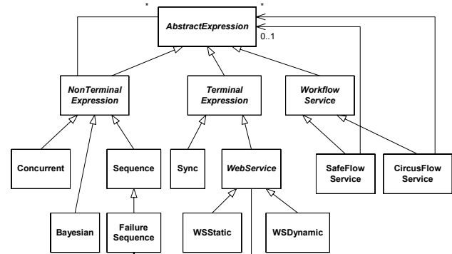
Figure 2 Language Design
