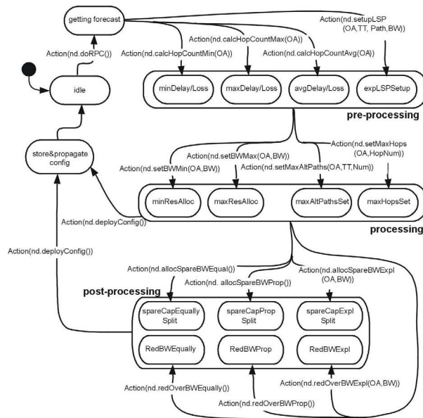
Figure 1: Network Dimensioning module behaviour.
