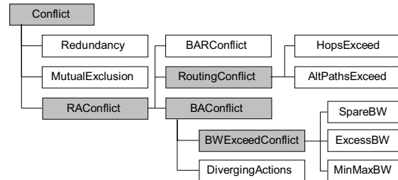
Figure 2: ND conflict classification.
