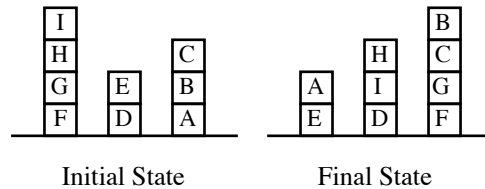
Figure 2: Blocks World Problem bw-large-b
