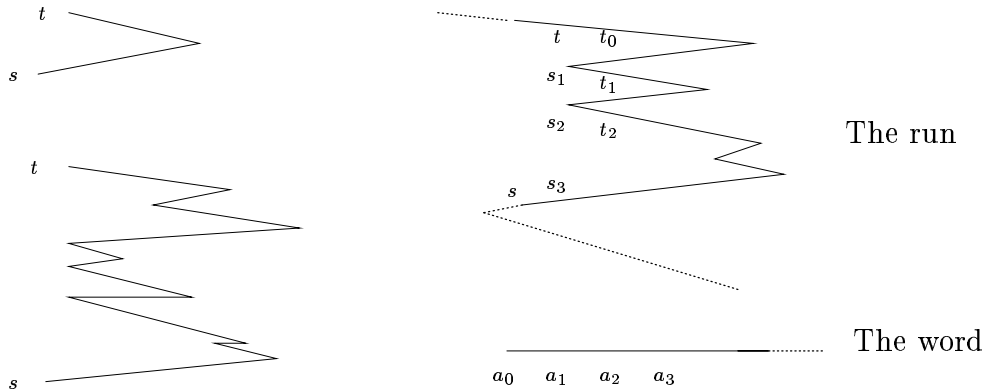
Figure A.2: (a) Different connecting segments (b) The transition at the pair state (t, s)
