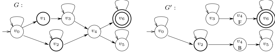
Figure 3: A colored Büchi graph G and the graph G' resulting from the transformation.
