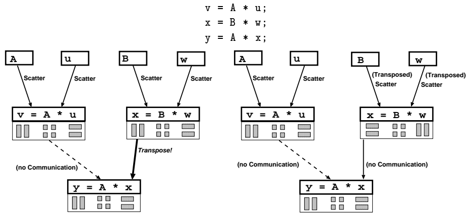
Fig. 1. Unoptimised (left) and optimised DAG for our example
