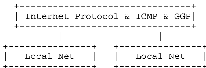
Gateway Protocols
