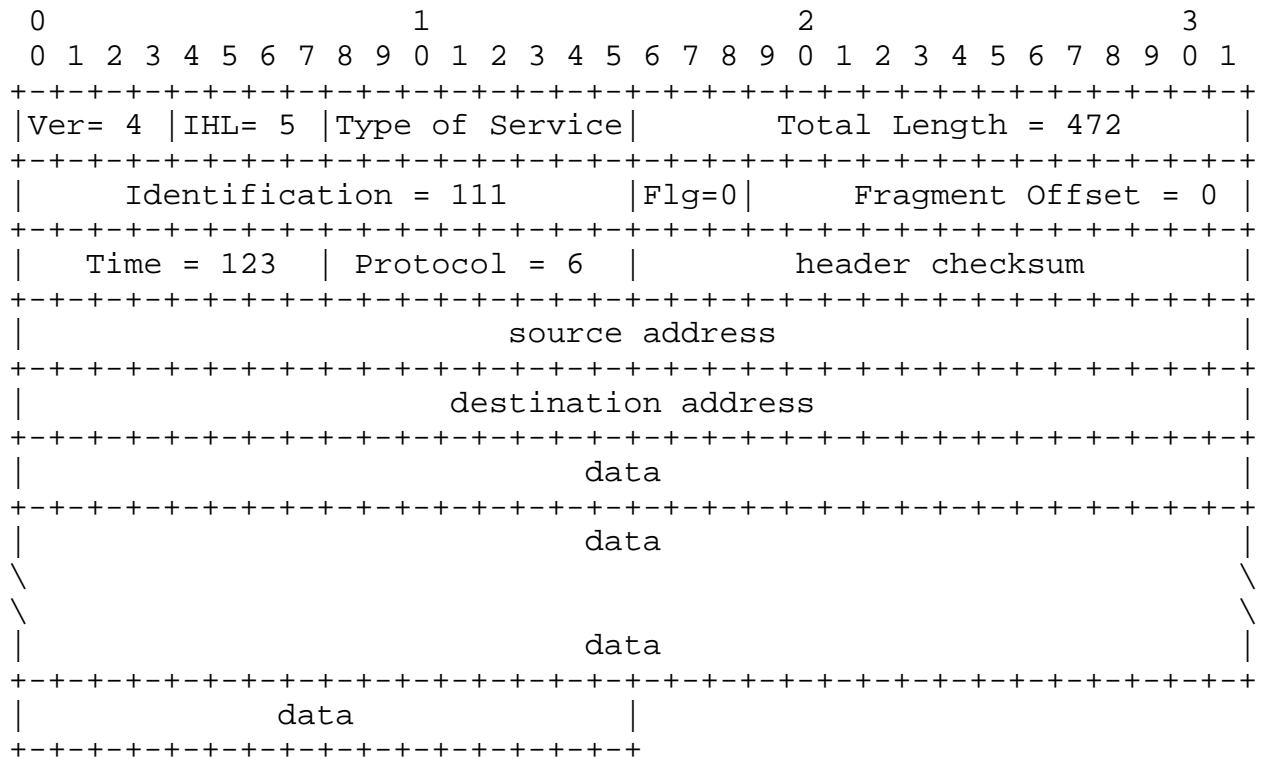
Example Internet Datagram
