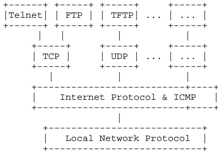
Protocol Relationships
