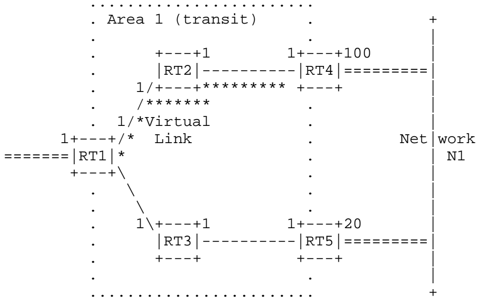
Figure 17: Routing through transit areas
