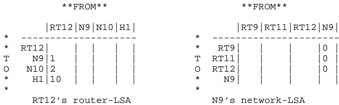
Figure 4: Individual link state components
