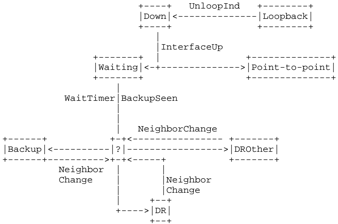
Figure 11: Interface State changes
