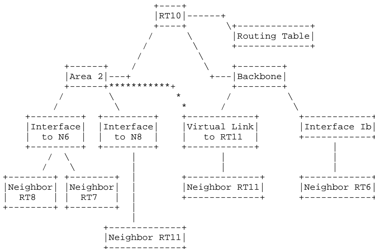
Figure 9: Router RT10's Data structures
