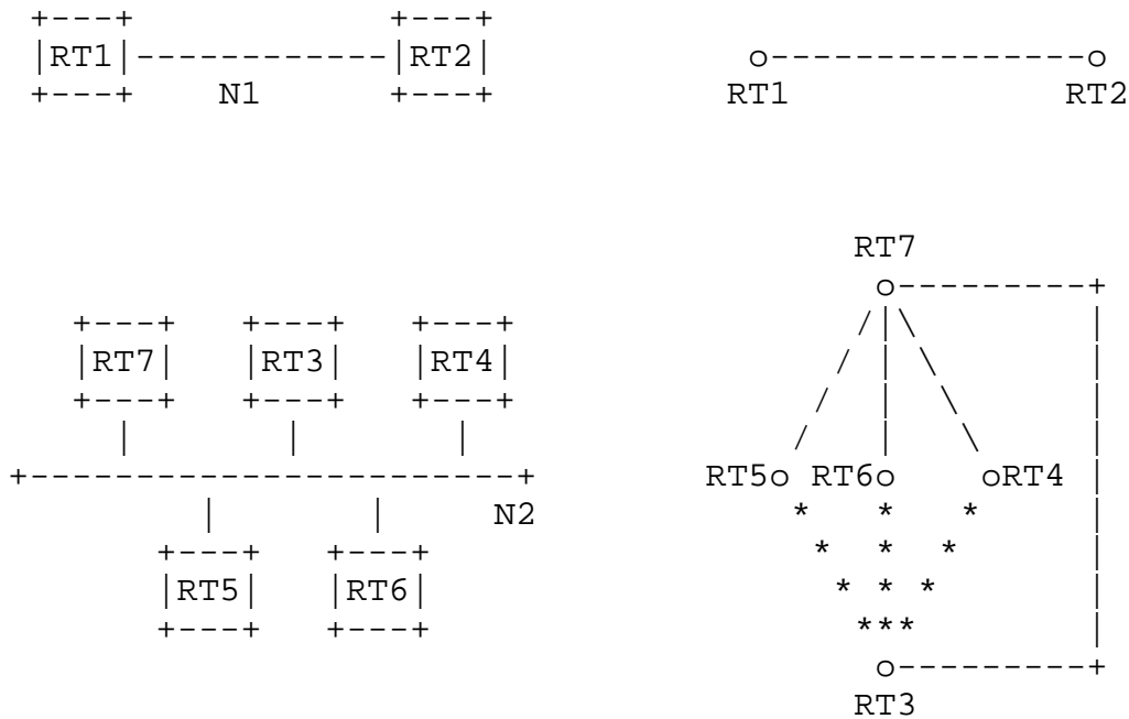
Figure 10: The graph of adjacencies
