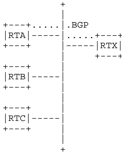
Figure 16: Forwarding address example
