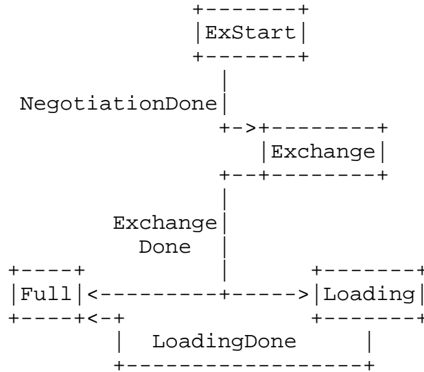
Figure 13: Neighbor state changes (Database Exchange)
