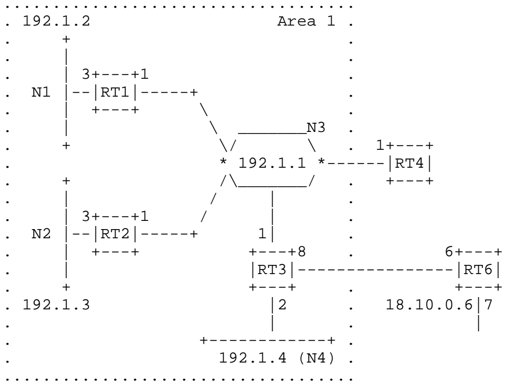
Figure 15: Area 1 with IP addresses shown
