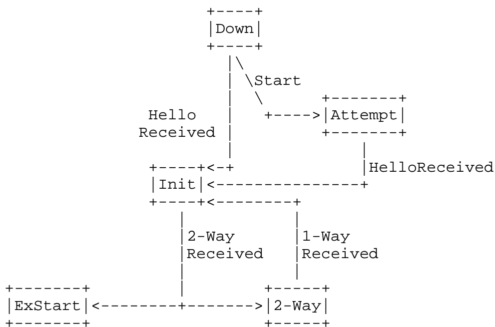
Figure 12: Neighbor state changes (Hello Protocol)
