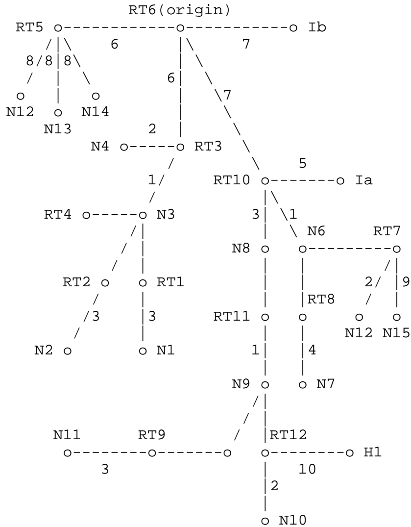
Figure 5: The SPF tree for Router RT6
