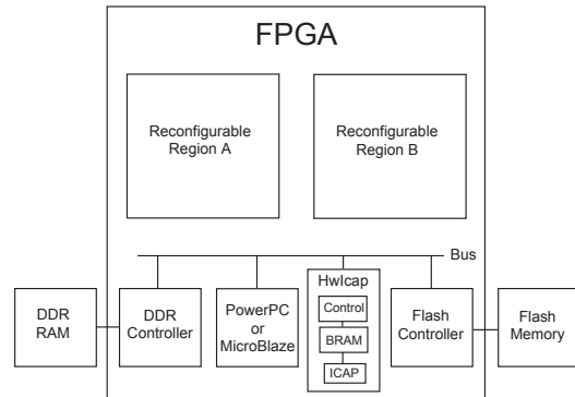
Figure 8. Example of a self-reconfigurable system with HwIcap.
