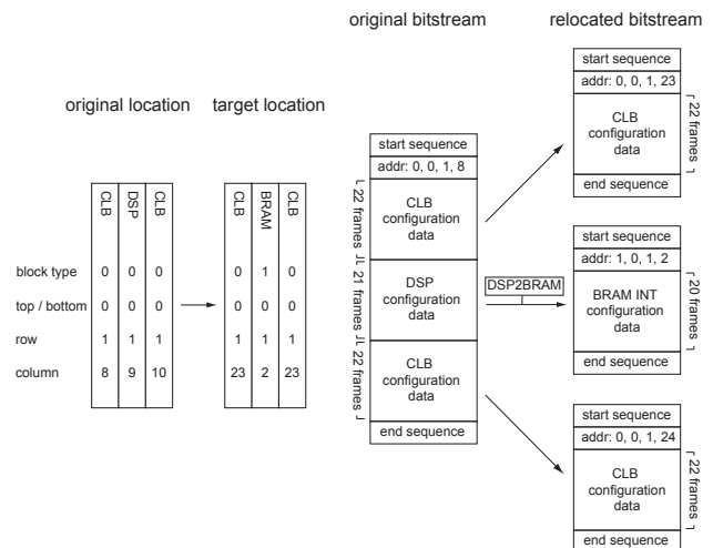
Figure 9. Example of a bitstream relocation from DSP to BRAM.
