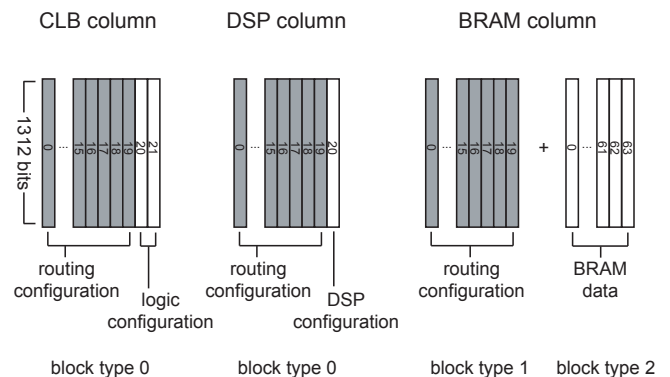
Figure 7. Configuration memory of CLB, DSP and BRAM resources.
