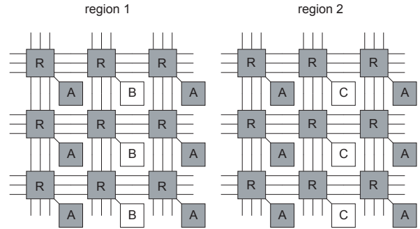
Figure 3. Heterogeneous FPGA fabric with compatible subset of resources.
