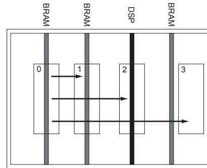
Figure 1. Relocation from region 0 to an identical (1) and non-identical regions (2, 3).
