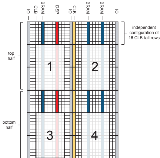
Figure 5. Structure of the Virtex4 LX25 FPGA with an exemplary floorplan of four reconfigurable modules.
