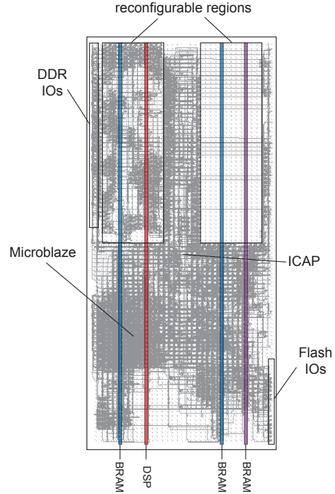
Figure 10. Reconfigurable and relocatable software defined radio prototype: filter for two audio channels on a Virtex-4 LX25 FPGA. A filter is implemented only in the left region and one bitstream is stored. The configuration can be relocated dynamically.
