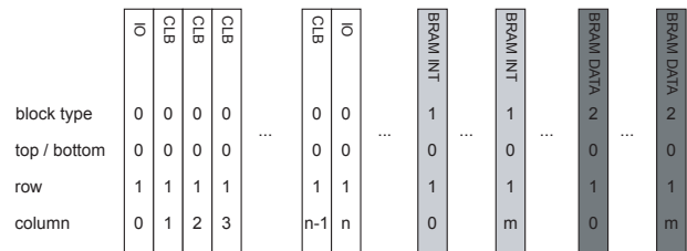
Figure 6. Configuration memory map in Virtex-4 FPGAs.
