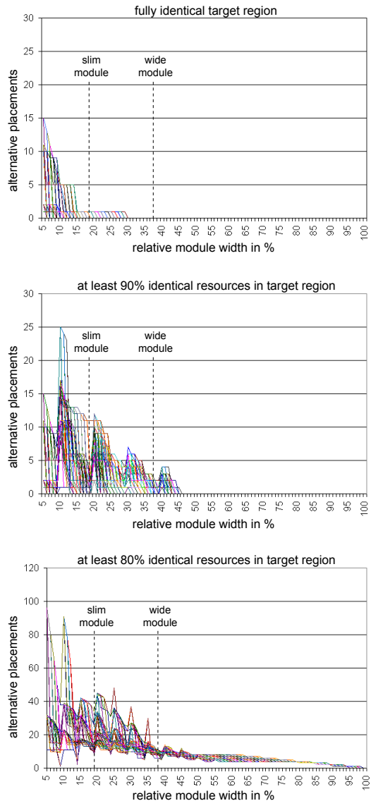
Figure 11. Alternative placement options for software defined radio application on an Virtex-4 FX140 FPGA for different relative module widths and for fully identical, at least 90% identical and at least 80% identical target regions.
