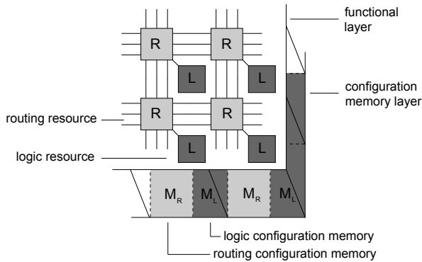
Figure 2. FPGA model with functional layer and configuration memory layer.
