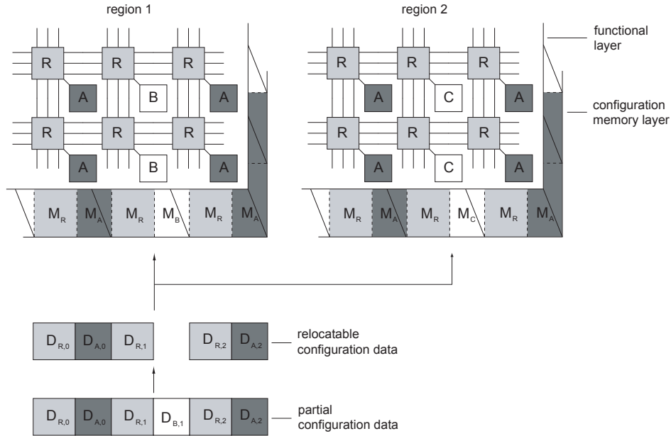
Figure 4. Model of a relocatable bitstream: configuration data corresponding to the compatible subset can be loaded in both locations.
