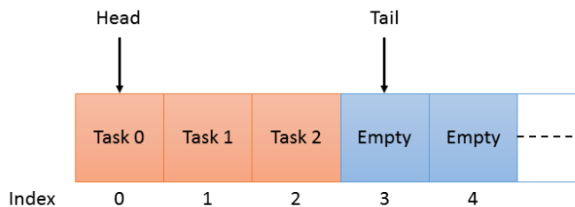
Figure 4.9. Example configuration of the concurrent deque
