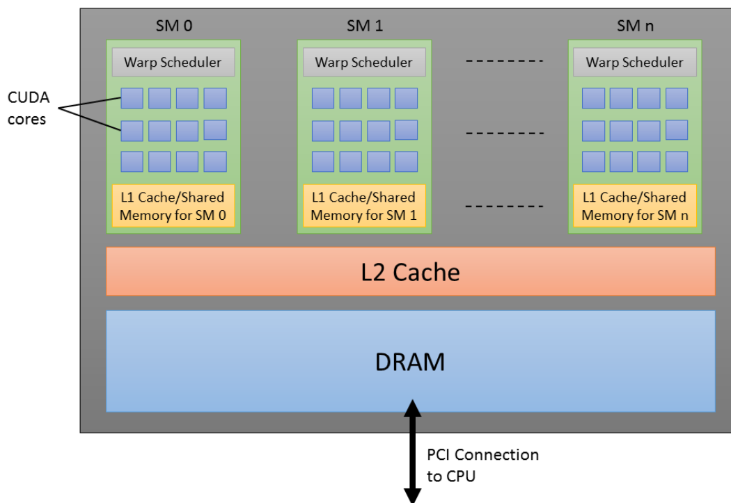
Figure 2.3. GPU hardware showing CUDA cores, SMs, and the memory hierarchy
