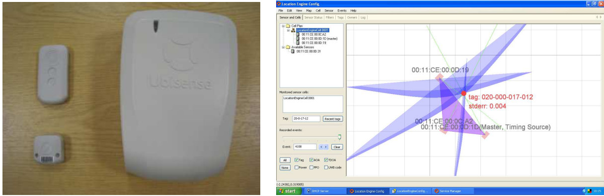
Figure 1: UWB-based sensors and tags (left) use a combination of angle-of-arrival and timed-difference-of-arrival triangulation schemes to enable high-accuracy tag location tracking (right)
