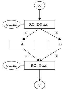
Fig. 10. A design that can behave either as A or as B , depending on the value of the input wire cond connected to the control blocks RC_DMux and RC_Mux .
