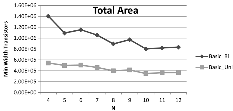
Fig. 10. FPGA area as N increases.
