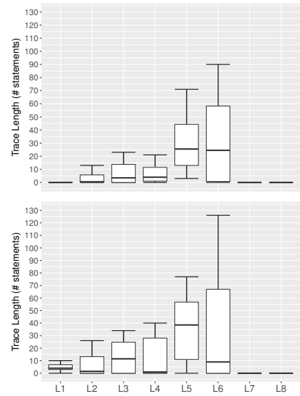
Figure 7: Trace length of the warnings reported at each layer in CHEETAH with SPB (top) and SPS (bottom).
