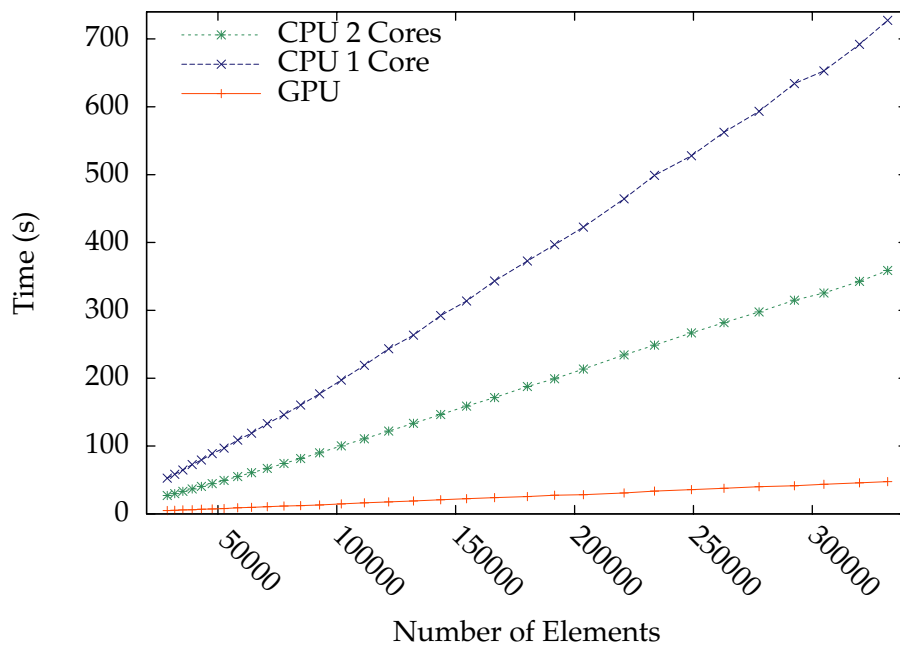
Figure 4.17: Time taken by the assembly phase in running the Advection system for 200 timesteps.
