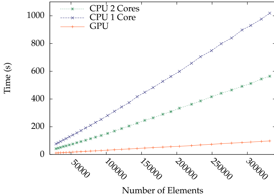
Figure 4.21: Total time running the Advection-Diffusion system for 200 timesteps.
