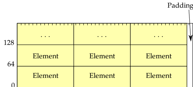
Figure 3.2: Padding of packed multiple elements to 64 bytes. From [Klößner et al. , 2009].
