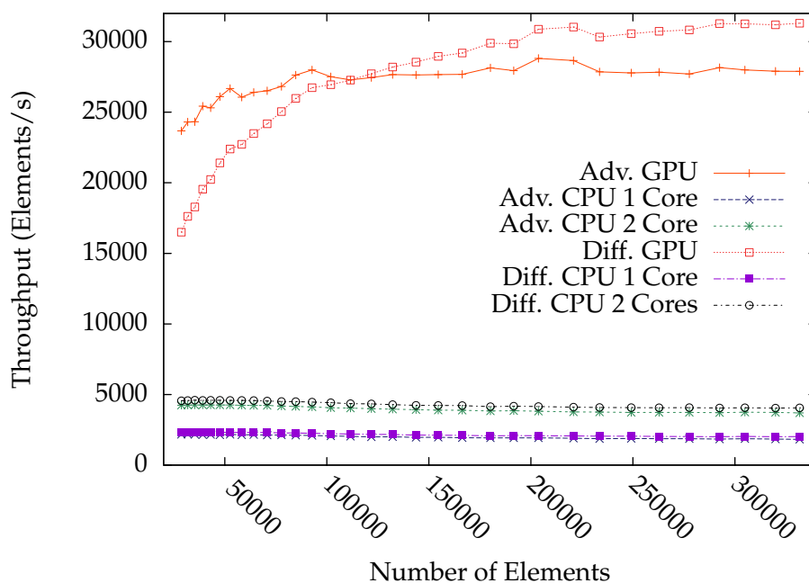
Figure 4.20: Throughput of assembly phase for each architecture and problem.
