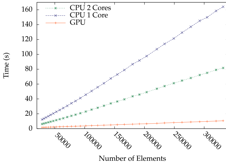
Figure 4.23: Total time running the Diffusion system for 200 timesteps.
