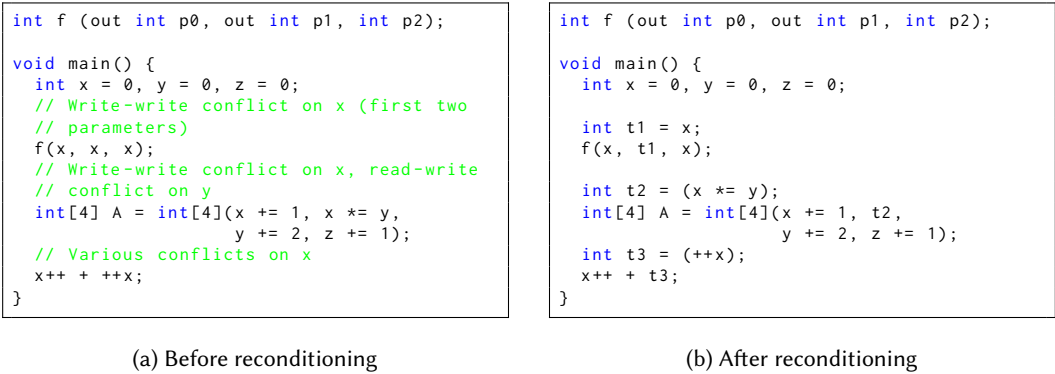
Fig. 4. Reconditioning to avoid undefined behaviour related to evaluation order
