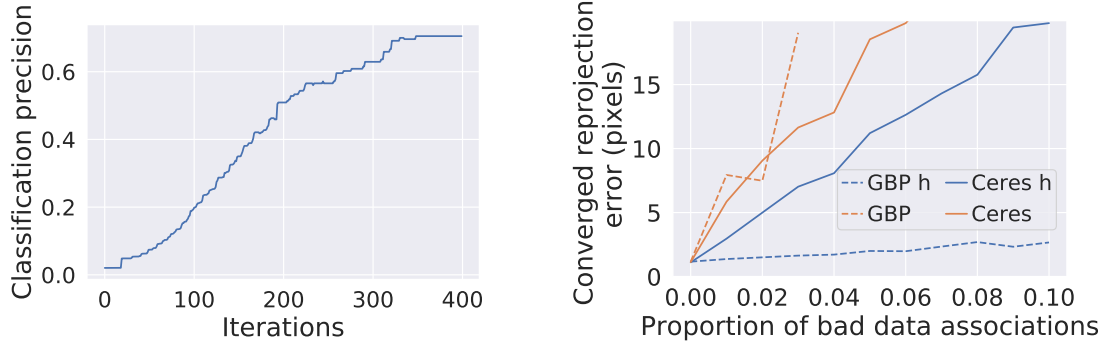
(a) Measurements are classified as outliers if they are in the linear loss regime. The recall is 1 over all iterations. ARE converges to < 1.5 pixels after 268 iterations while the precision is still increasing.
