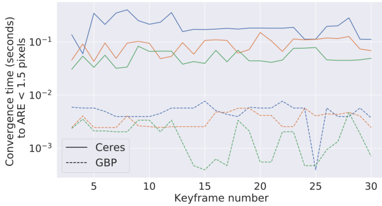
(b) SLAM. Time to converge to \text{ARE} < 1.5 pixels after a new keyframe is added and initialised with the pose of the most recent keyframe. Results are for the first 30 keyframes of the sequences fr1desk , fr2desk , fr3teddy .
