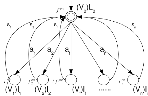
Fig. 3. Mapping between an OWL-S atomic process and ISPL
