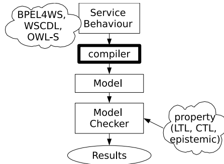
Fig. 1. General architecture for service verification
