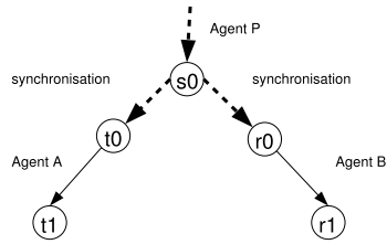
Fig. 9. Encoding choice
