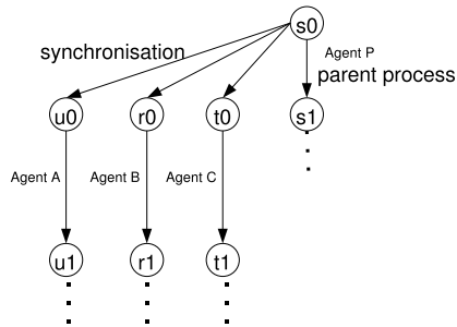
Fig. 6. Encoding split
