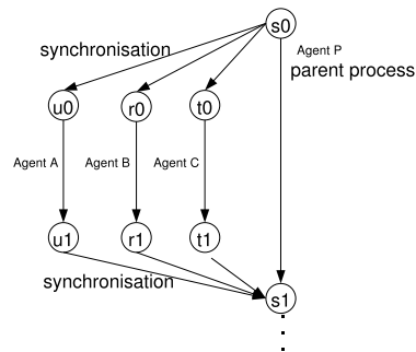
Fig. 7. Encoding split+join
