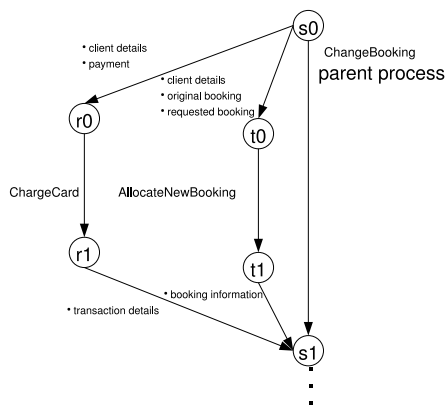
Fig. 8. The ChangeBooking process
