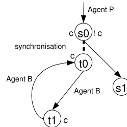
Fig. 12. Encoding repeat-while-repeat-until
