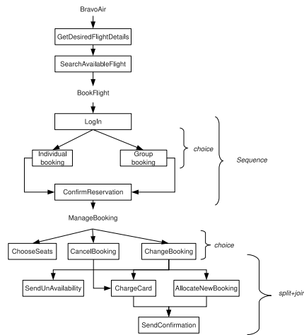
Fig. 2. An extended version of the BravoAir process
