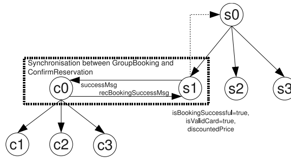
Fig. 5. Sequential composition of GroupBooking and ConfirmReservation
