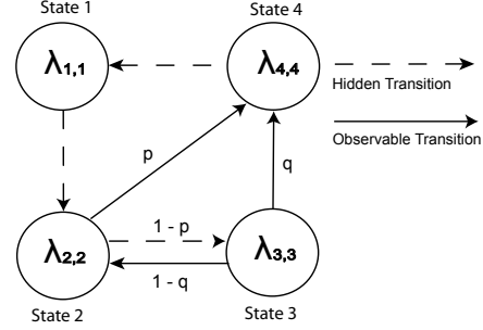
Figure 1. Example of Markovian Arrival Process (MAP)
