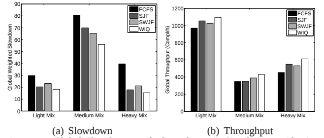
Figure 5. Global Slowdowns and Throughputs in Simulations with First-Come First-Served (FCFS), Shortest-Job-First (SJF), Shortest-Weighted-Job-First (SWJF), and Work-Intensive-Query First (WIQ) Scheduling.
