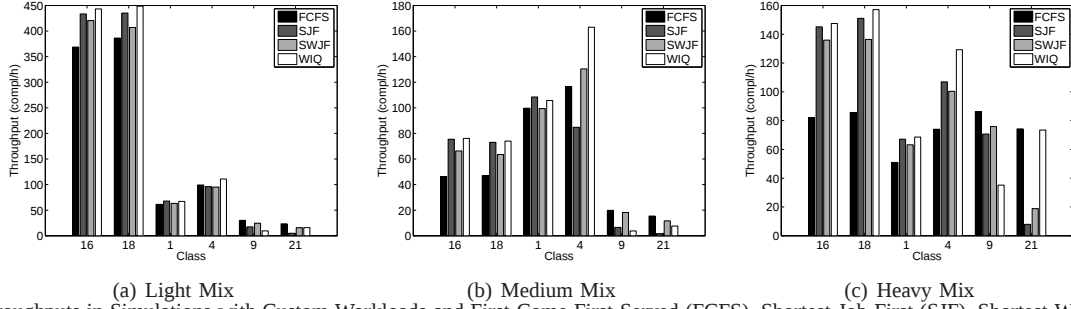
Figure 6. Throughputs in Simulations with Custom Workloads and First-Come First-Served (FCFS), Shortest-Job-First (SJF), Shortest-Weighted-Job-First (SWJF), and Work-Intensive-Query First (WIQ) Scheduling.
