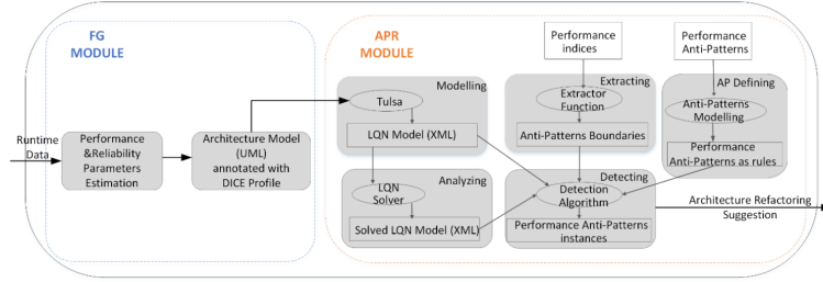
Fig. 2. DICE enhancement tool workflow.
