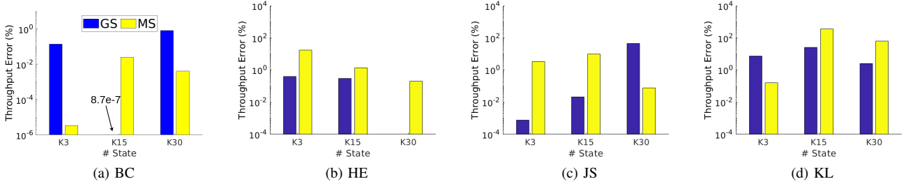
Fig. 3: Divergence comparison with 10 clients using GS and MS algorithms.
