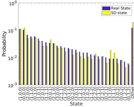
Fig. 5: State probability distribution for the model with K30 state and 10 clients.
