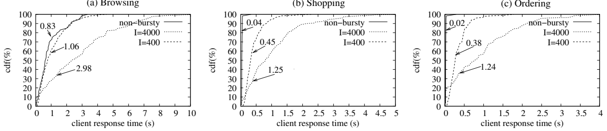
Figure 6: CDFs of latencies for (a) browsing mix, (b) shopping mix, and (c) ordering mix with non-bursty and bursty of I = 4000 and 400 in user think times, where N = 1000 and the corresponding average latencies are also marked.
