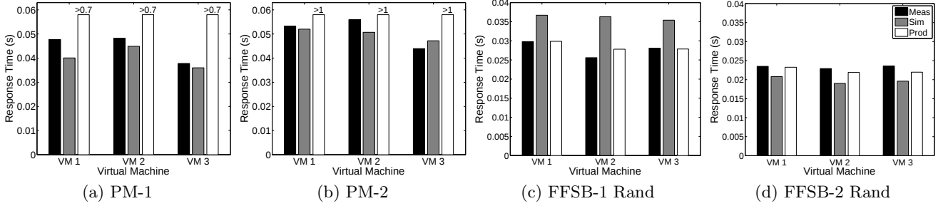
Figure 10: Comparison of Response Times from Measurement (Meas), Simulation (Sim), and Product-Form (Prod) Model for Three VMs Consolidation Scenarios With Largest Prediction Errors. Legend Shown in Figure (d) is Identical for Figures (a), (b) and (c).
