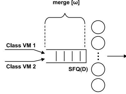
Figure 5: Queueing Model.
