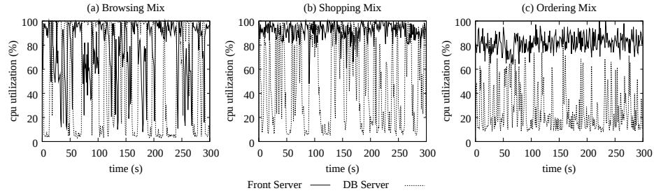
Fig. 5. The CPU utilization of the front server and the database server across time with 1 sec granularity for (a) the browsing mix, (b) the shopping mix, and (c) the ordering mix under 100 EBs. The monitoring window is 300 seconds.
