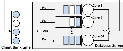
Fig. 4. Multiclass Fork-Join Queueing Model of a Database Server as follows [10]:
