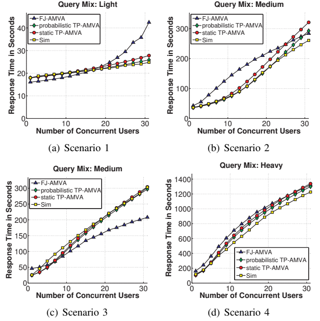
Fig. 5. Response Time Results under OLAP-based Workloads
