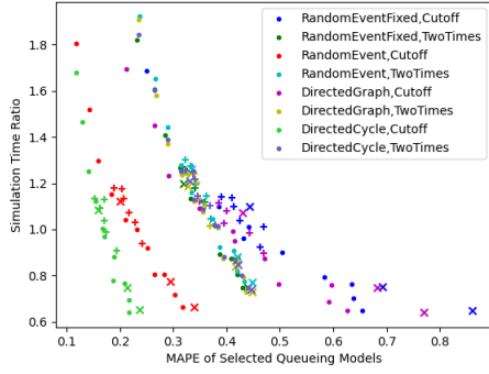
Figure 2: MAPE vs Simulation Time Ratio under different \tau formulas. Markers + : k/\max(a_j) , \circ : k/\text{avg}(a_j) , \times : k/\min(a_j)
