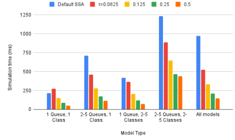
Figure 3: Simulation Time (ms) under different values of \tau , by model type
