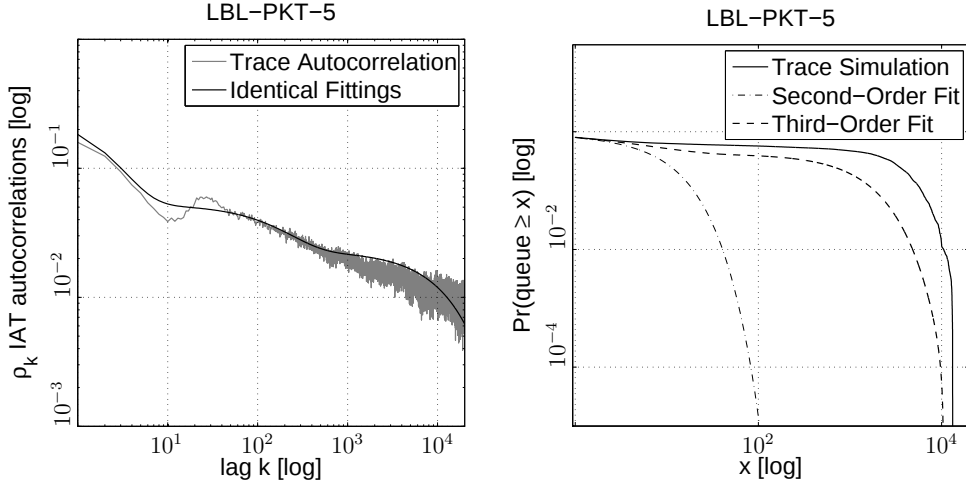
Fig. 1. Autocorrelation and MAP/M/1 queueing behavior (util. 80%) of two MAP(32) fittings of the LBL-PKT-5 trace [1]. The MAPs have identical first and second order properties of the interarrival process, but one has also an accurate fitting of third order properties for which the other is instead loose.
