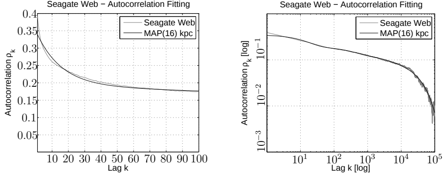
Fig. 8. Fitted autocorrelation for the Seagate Web trace using the program in Figure 2.
