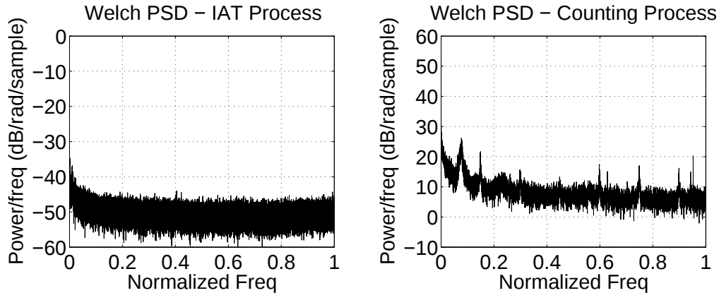
Fig. 4. Comparison of the power spectrum of the IAT process and the counting process for the Bellcore Aug89 trace. The counting process shows power density in the complex spectrum which is instead negligible in IATs.
