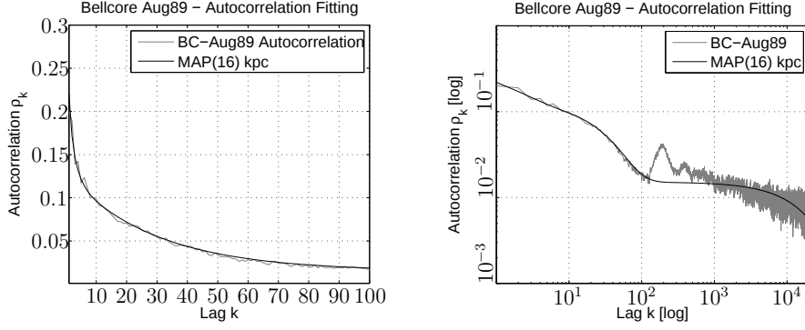
Fig. 5. Fitted autocorrelation for the Bellcore Aug89 trace using the program in Figure 2.
