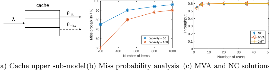
(a) Cache upper sub-model (b) Miss probability analysis (c) MVA and NC solutions Fig. 5. Capabilities of LINE in analyzing multi-formalism LQN models
