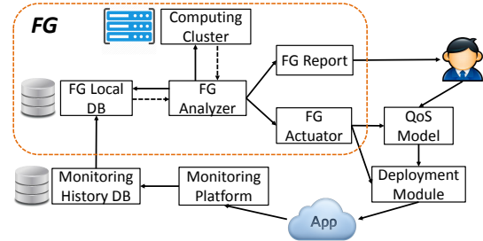
Figure 1: FG Architecture
