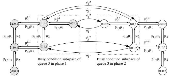
Figure 4: Underlying Markov process of the network in Figure 3 in the simple case when the MAP is a MMPP(2) process; the job population is N = 2 . Two queues are exponential with rates \mu_1 \equiv \mu_1^{1,1} and \mu_2 \equiv \mu_2^{1,1} , respectively; the third queue is a MAP with K_3 = 2 phases having \mu_3^{k,h} = 0 for k \neq h , that is a MMPP(2) process. (002, 1) indicates that the exponential queues are idle and the MAP queue has two jobs and is in phase 1; in (110, 2), the phase 2 is the phase left active by the last served job.
