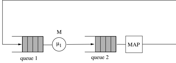
Figure 1: Example model with nonrenewal service. The service is an exponential process with rate \mu_1 at queue 1, at queue 2 is a possibly nonrenewal two-phase Markovian Arrival Process (MAP(2)) [28].
