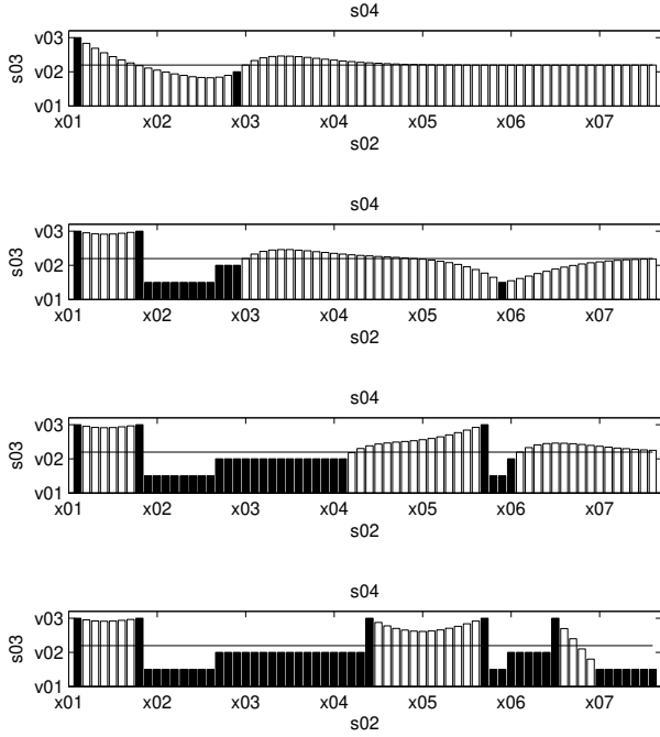
Figure 3: Intermediate steps of CWS execution on the case study. Legend: \square = expected job size (i.e., E[S_j|m] ), \blacksquare = observed job size (i.e., S_j ), - is the mean job size (i.e., E[S] = 1.2 ).
