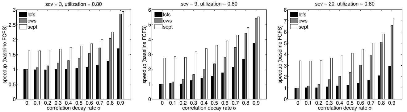
Figure 7: K = 3 workload classes: comparison of CWS, LCFS, and SEPT speedups over FCFS, window size W = 10^4 .
