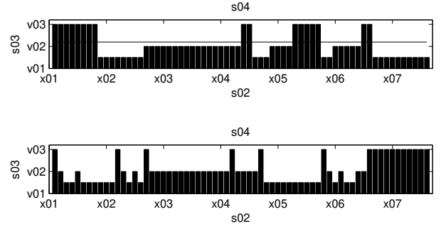
Figure 4: Case study of a workload with 65 jobs sampled from three classes with deterministic distribution and means 0.5, 1, and 2. The horizontal line in figure (a) is the mean job size E[S] = 1.2 .
