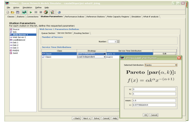
Figure 5: JSIMwiz - Wizard-guided analysis
