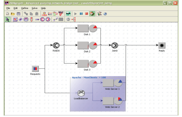
Figure 3: JSIMgraph - Graphical design workplace
