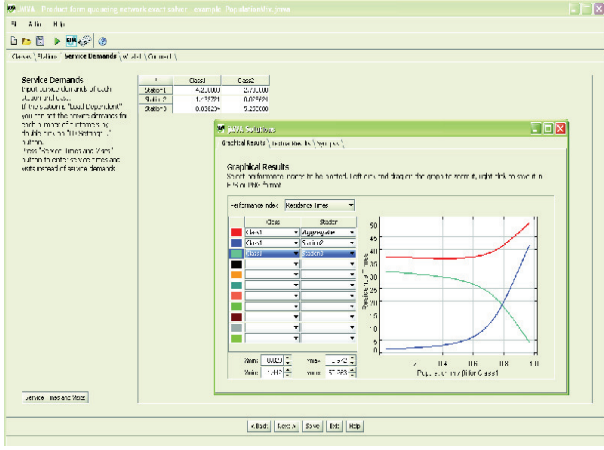
Figure 6: JMVA - What if analysis
