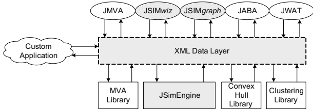
Figure 1: JMT - General Architecture
