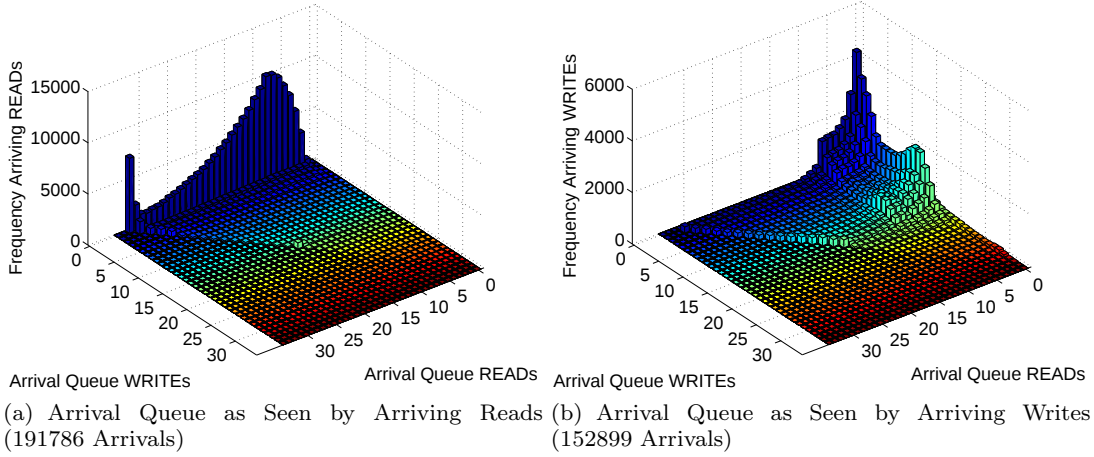
Fig. 10 Arrival Queue Lengths From a Two VM Consolidation Experiment (Web+Mail).
