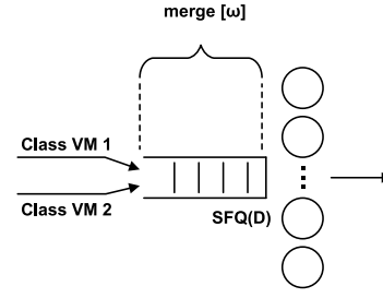
Fig. 5 Queueing Model.
