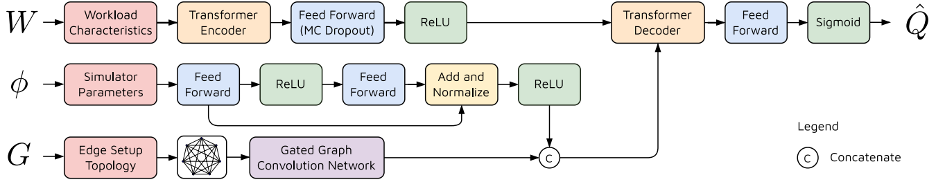
Figure 3. Low-Fidelity surrogate of the simulator in SimTune in the form of a neural network. The inputs include workload characteristics as time-series values, simulator parameters and edge topology as a fully-connected graph. The output is a vector of QoS estimates.
