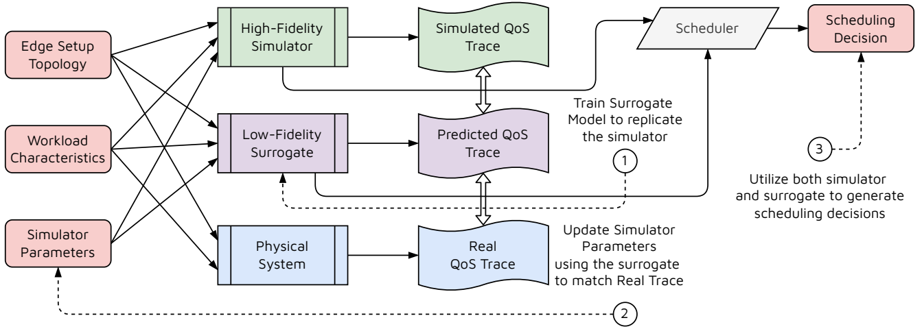
Figure 2. SimTune Pipeline
