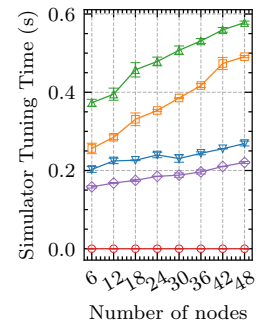
Figure 6. Tuning time of SimTune and baseline models with different number of nodes in the edge-cloud setup.
