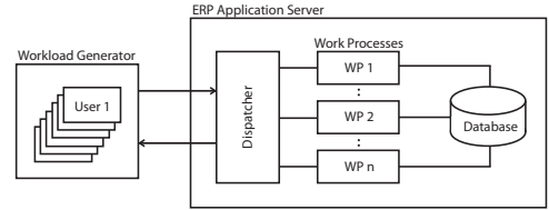
Figure 1: SAP application server architecture.
