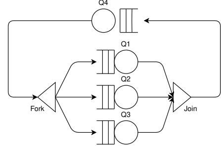
Figure 1: Queueing network containing a fork-join system
