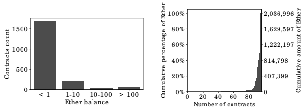
(a) Ether held by contracts in our dataset with non-zero balance. (b) Cumulative Ether held in the 96 contracts in our dataset containing at least 10 ETH.
