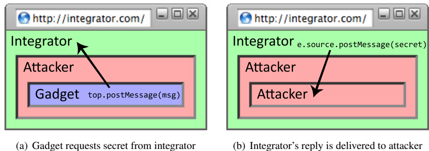
Figure 5: Reply Attack
