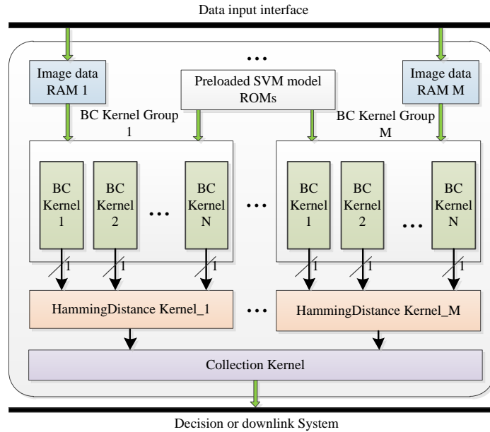
Fig. 1. Architecture of multi class classifier for HSI classification
