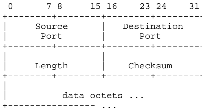
User Datagram Header Format
